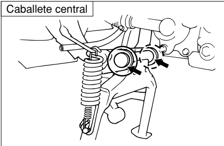
Caballete central
