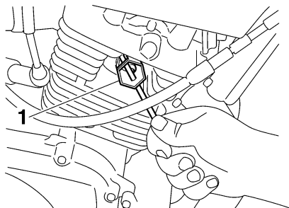
1. Zündkerzenschlüssel
