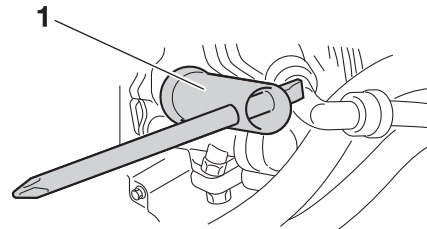
1. Zündkerzenschlüssel
